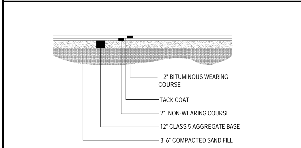
BITUMINOUS TURN LANE SECTION
