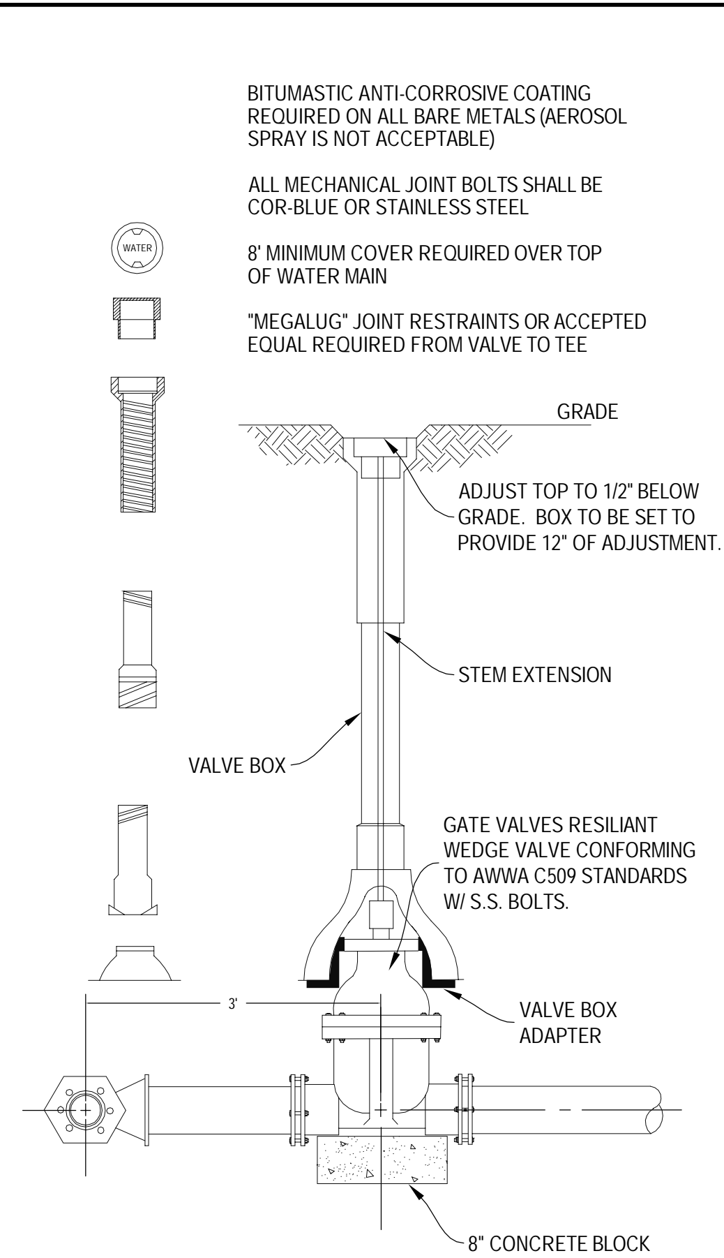
GATE VALVE AND BOX INSTALLATION
