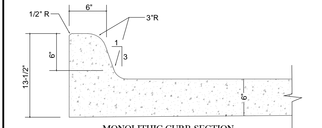
MONOLITHIC CURB SECTION
