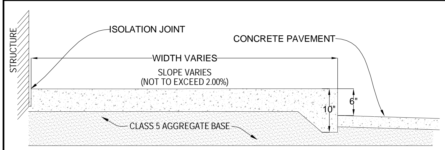
CONCRETE INTEGRAL SIDEWALK DETAIL
