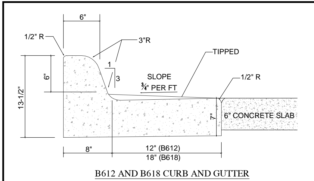
B612 AND B618 CURB AND GUTTER
