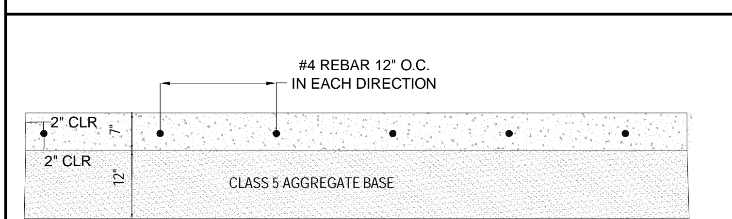
TYPICAL CONCRETE SECTION OVER U.G.S.T. AREAS
